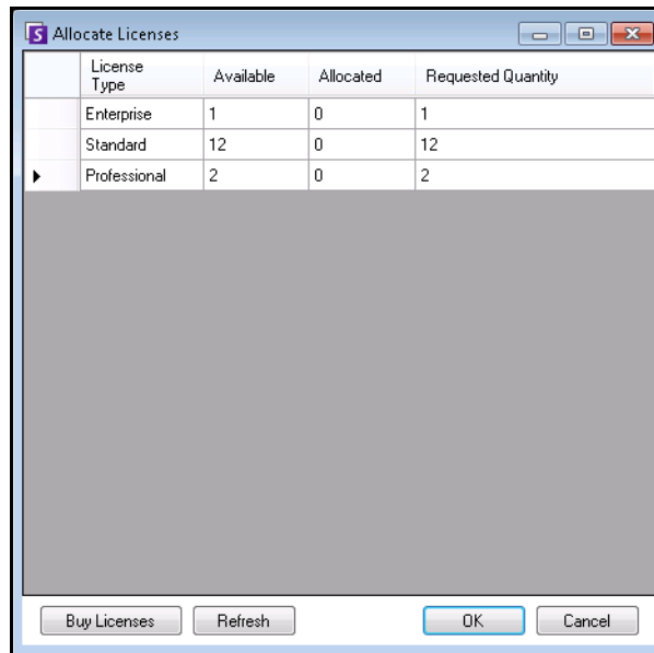
Figure 13. Allocate licenses
