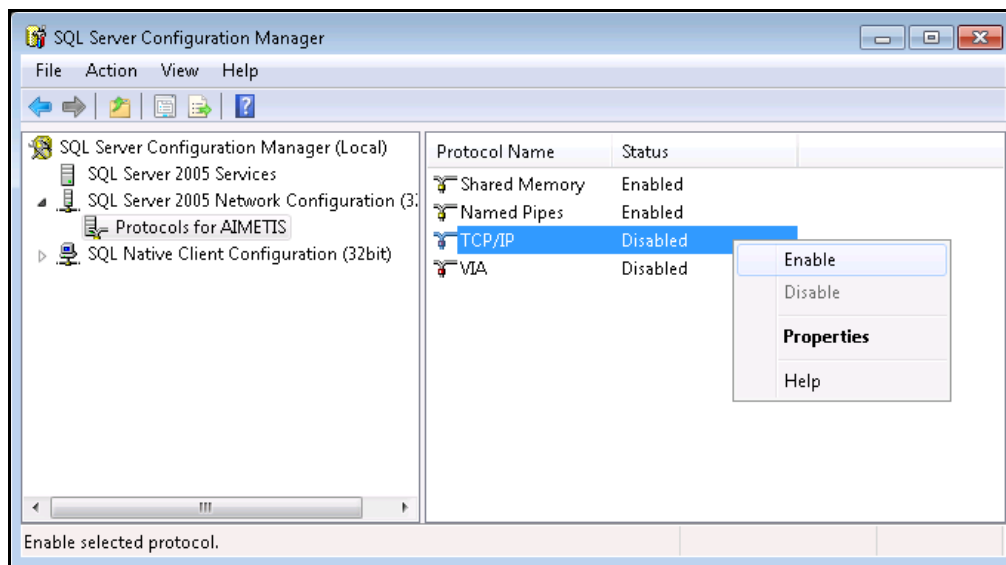
Figure 8. Enable TCP/IP
