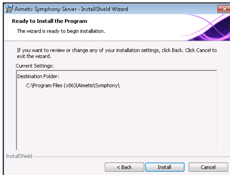
Figure 5. Destination folder
