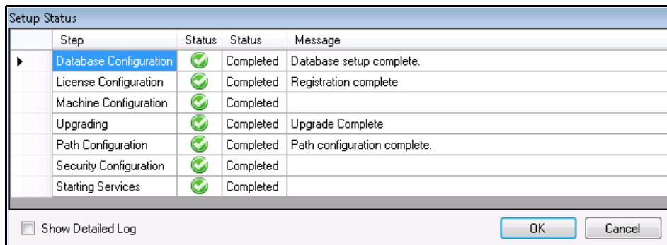
Figure 20. Setup Status
